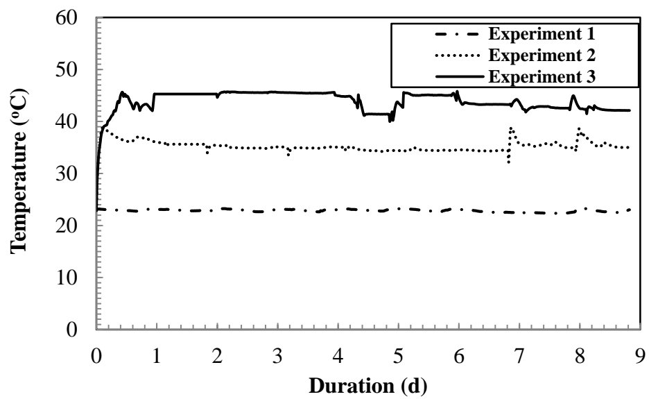
Figure 4-2. Temperature profile during the experimental runs
