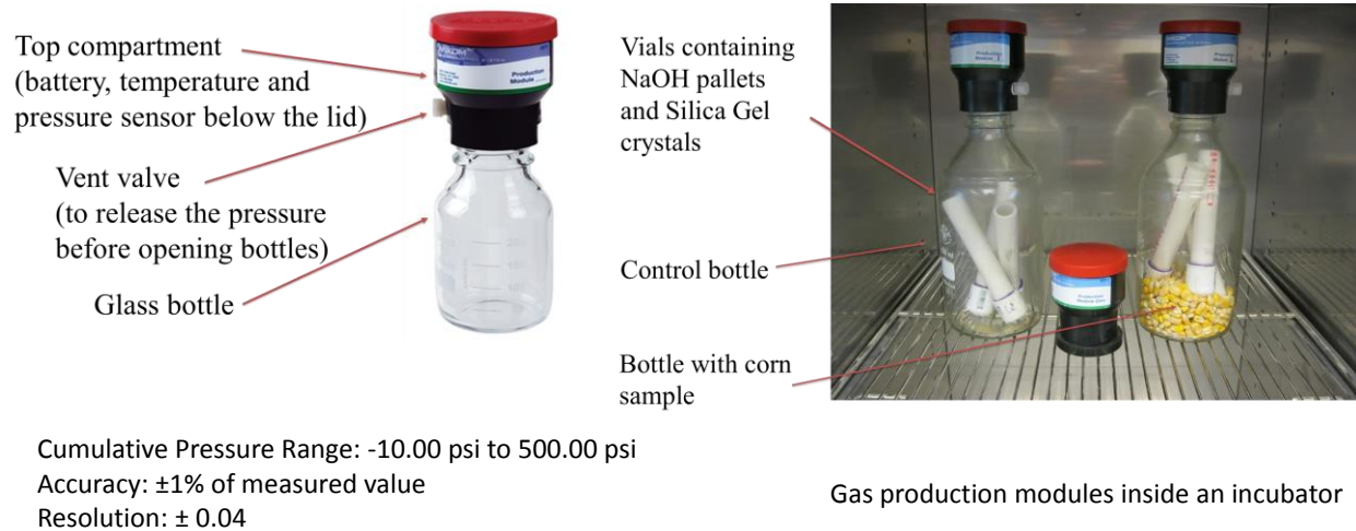
Figure 3-1. Experimental setup.
