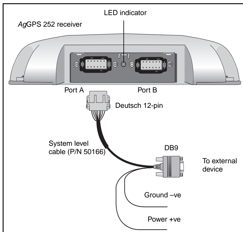
Figure 3.1 Standard power/data cable connections
